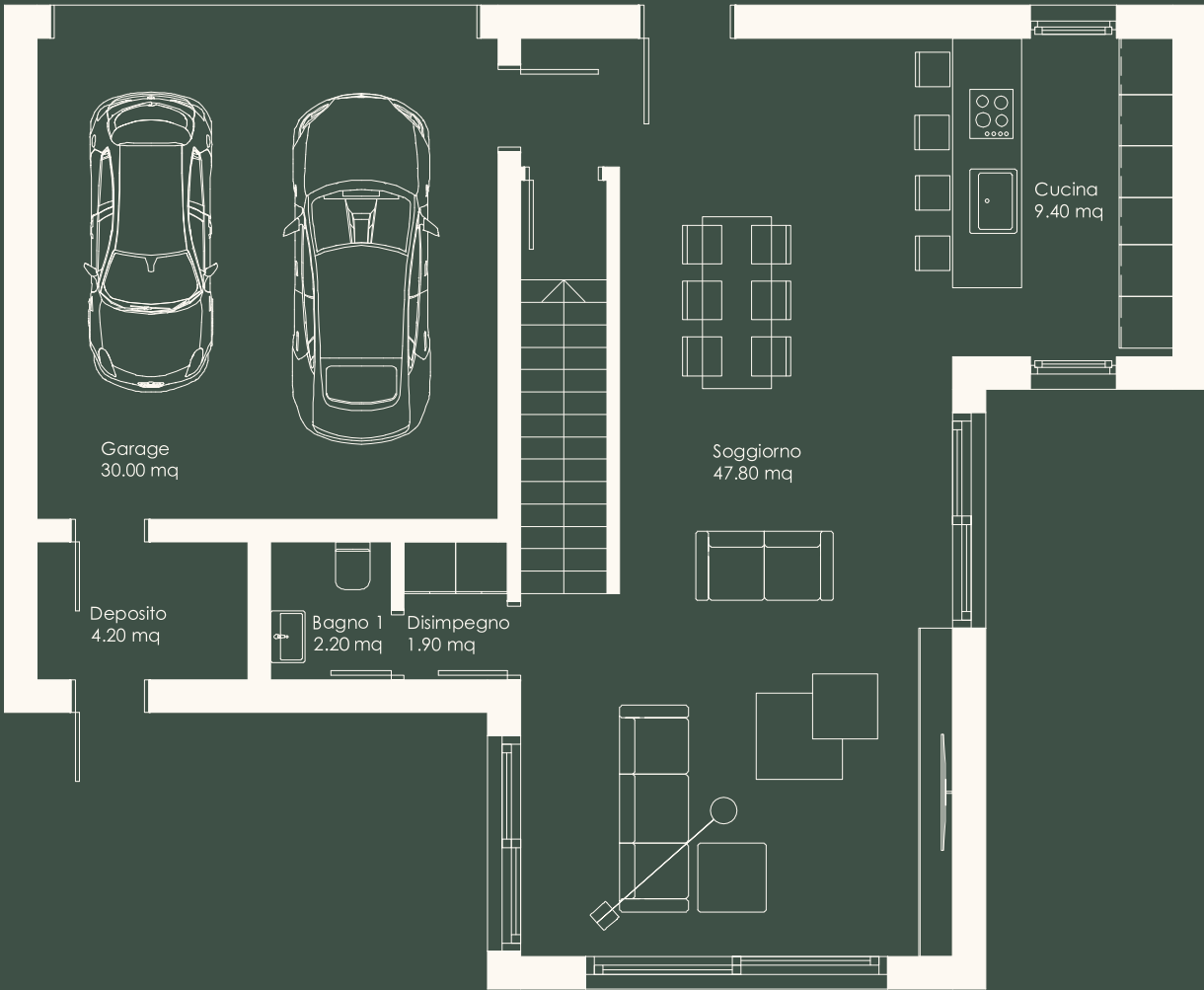
Piano terreno
